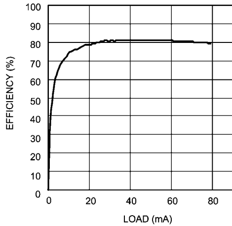
Efficiency vs Load Current - "Y" V_{IN} = 2.7V, V_{OUT} = 12V
